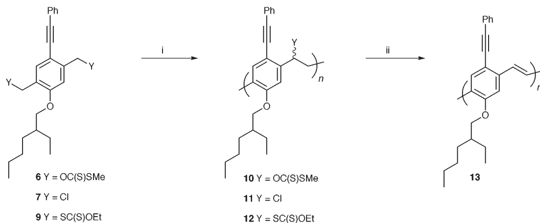
Scheme 2 Reagents and conditions: i, KOBu^t , THF, Ar; ii, heat, vacuum.
