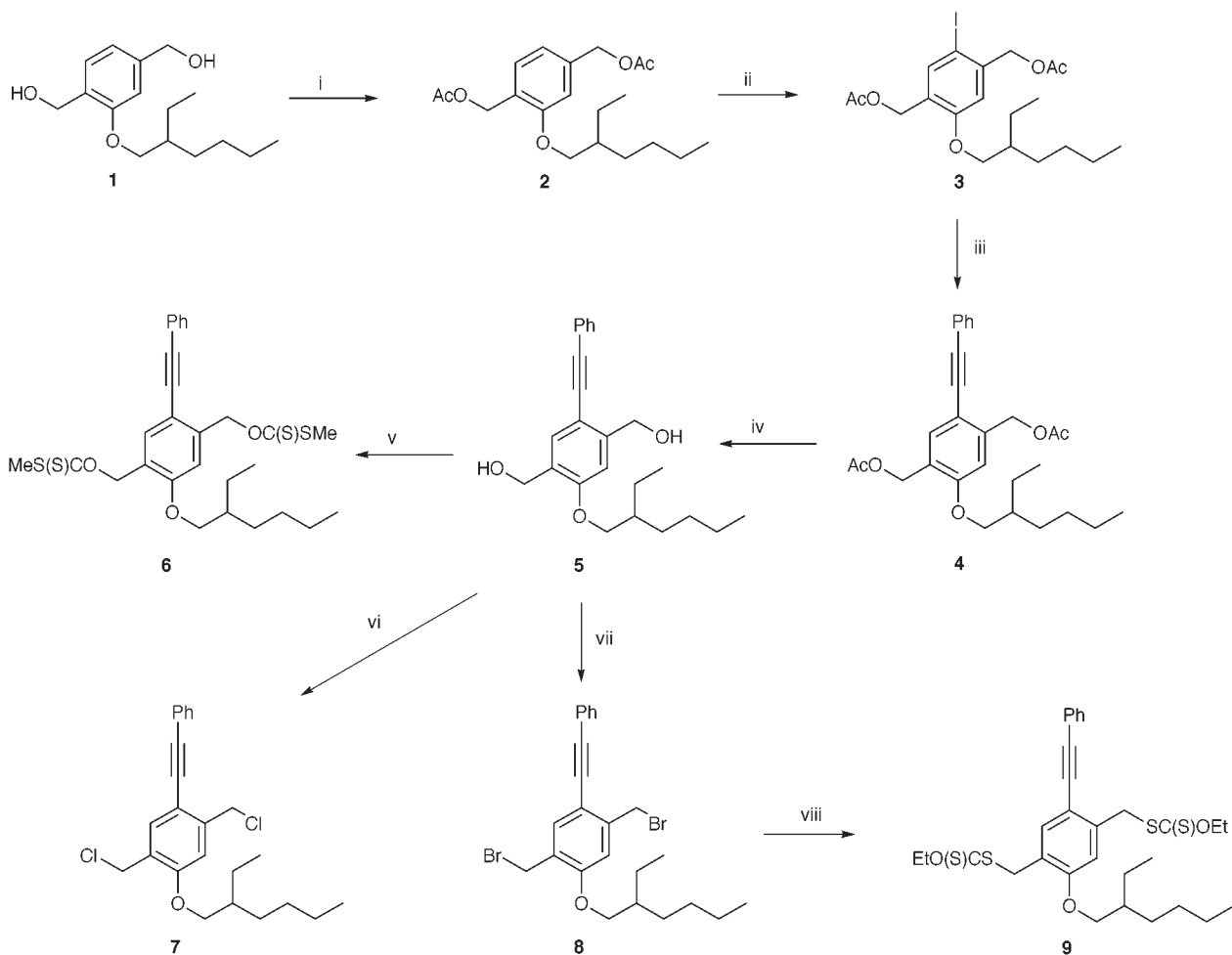
Scheme 1 Reagents and conditions: i, acetic anhydride, pyridine, heat, N_2 ; ii, I_2 , AgOAc, CHCl_3 , room temp.; iii, PhCCCu, pyridine, heat, N_2 ; iv, NaOH, H_2O , MeOH, CH_2Cl_2 , room temp., Ar; v, NaH, diethyl ether, heat, then CS_2 , heat, then MeI, heat, Ar; vi, DMAP, tosyl chloride, triethylamine, CH_2Cl_2 , room temp., N_2 ; vii, PBr_3 , diethyl ether, room temp., Ar; viii, potassium O -ethyl xanthate, ( n -Bu) _4 NBr, CH_2Cl_2 , Ar, room temp.
